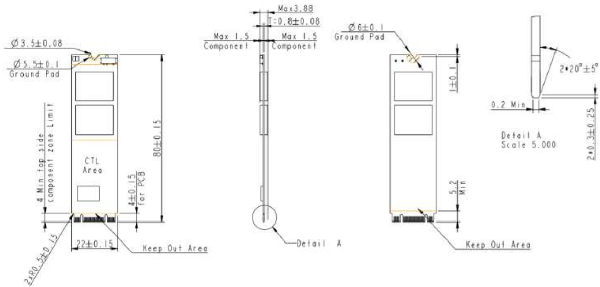
Figure 10-2 Dimensions – Double Side
